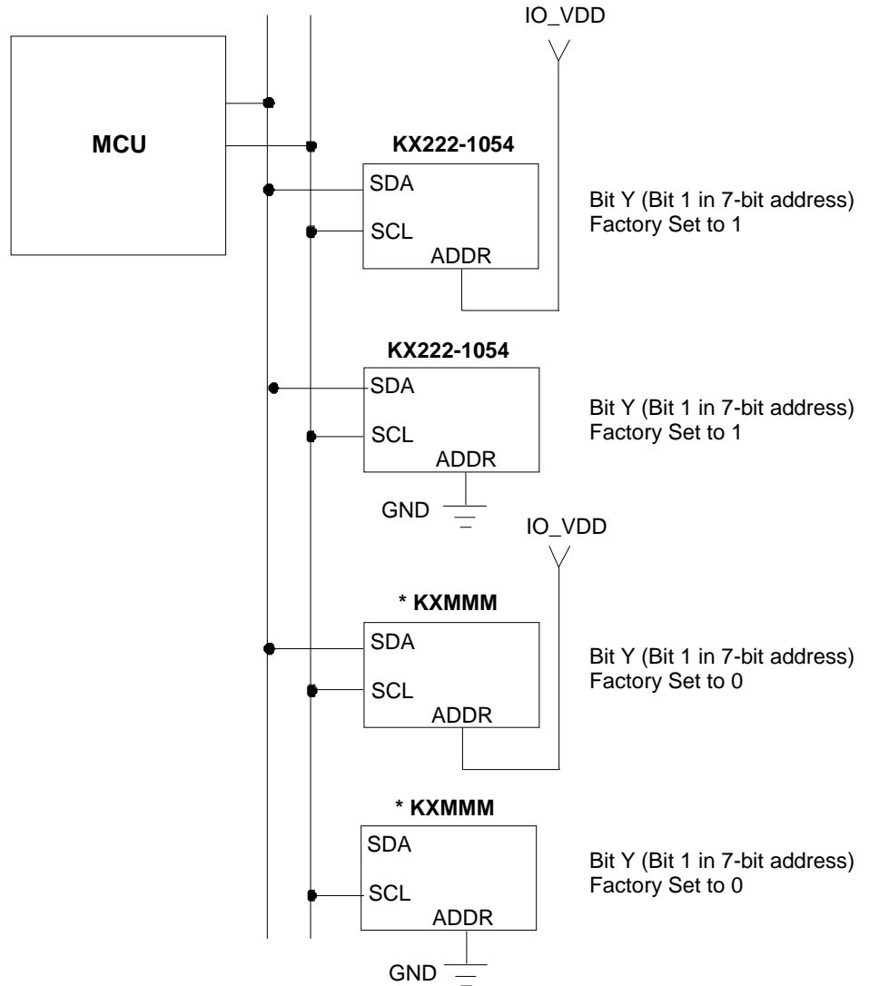
Figure 1: Multiple KX222 Accelerometers on a Shared I 2 C Bus
