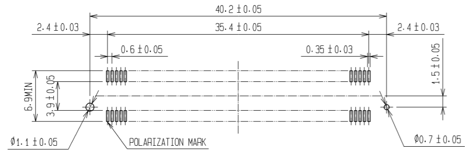
RECOMMENDED LAND PATTERN DIMENSION OF PCB (MOUNTING SIDE) (2:1) (RECOMMENDED METAL MASK THICKNESS:0.15mm)
