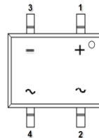
Pin Diagram
